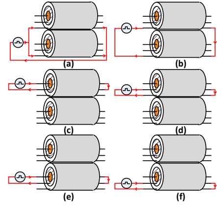
Fig. 5. Equivalent circuits for the modes in TCE-HVDC cables (a): ground (b): interarmor (c): coaxial 1 (d): sheath 1 (e): coaxial 2 (f): sheath 2.
