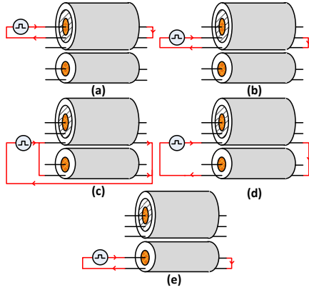
Fig. 4. Equivalent circuits for the modes in SCEMR-HVDC cables (a): coaxial (b): sheath (c): ground (d): interarmor (e): coaxial 2.
