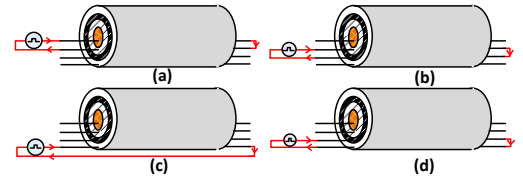
Fig. 6. Equivalent circuits for the modes in EIMR-HVDC cables (a): coaxial (b): sheath (c): ground (d): return.
