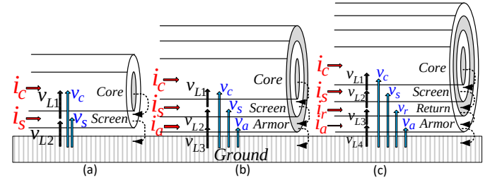
Fig. 2. Loops along cable layers for different HVDC cable constructions. (a): Two conducting layers cable (b): three conducting layers cable (c): Four conducting layers cable.
