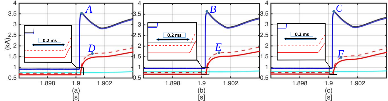
Fig. 12. Impact of the grounding scheme on the fault location in TCE-HVDC cable. (a) Two-sided bonded (b) Two-sided bonding + distributed grounding of armor (c) Two-sided bonding + distributed grounding of screen and armor
