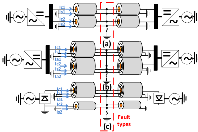
Fig. 8. Single line diagram and the involved layers in the faults for different cable bundles used in simulations (a): TCC-HVDC (b): TCE-HVDC (c): SCEMR-HVDC.
