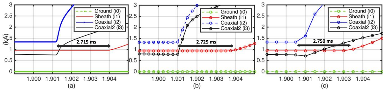
Fig. 9. Impact of sampling frequency on the modal fault location in TCC-HVDC cable. (a) 1 MHz, (b) 40 kHz, (c) 20 kHz
