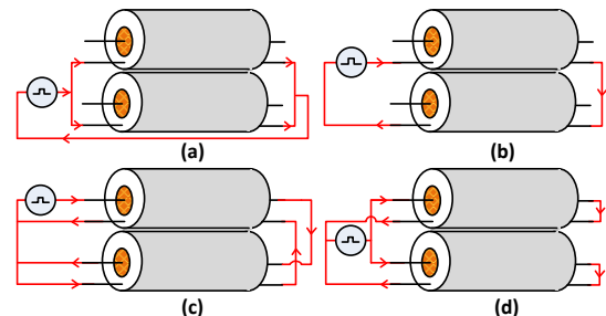
Fig. 3. Equivalent circuits for the modes in TCC-HVDC cables (a): ground (b): intersheath (c): coaxial 1 (d): coaxial 2.
