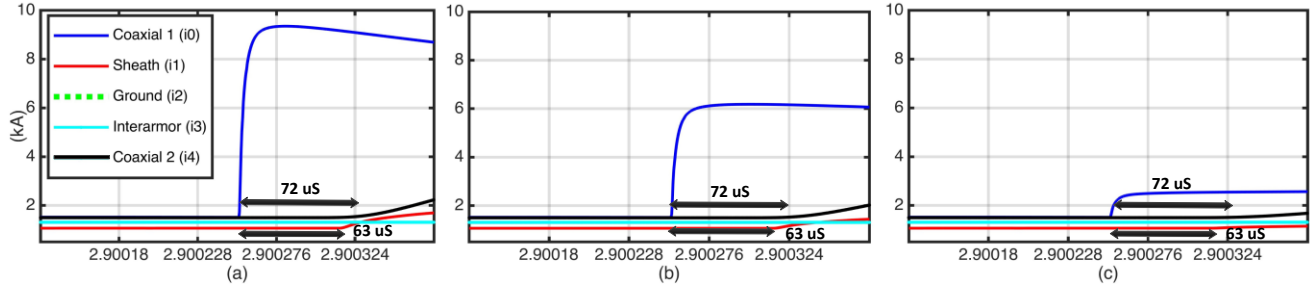
Fig. 10. Impact of fault resistance on the modal fault location in SCEMR-HVDC cable. (a) 0.1Ω (b) 1Ω (c) 100Ω.
