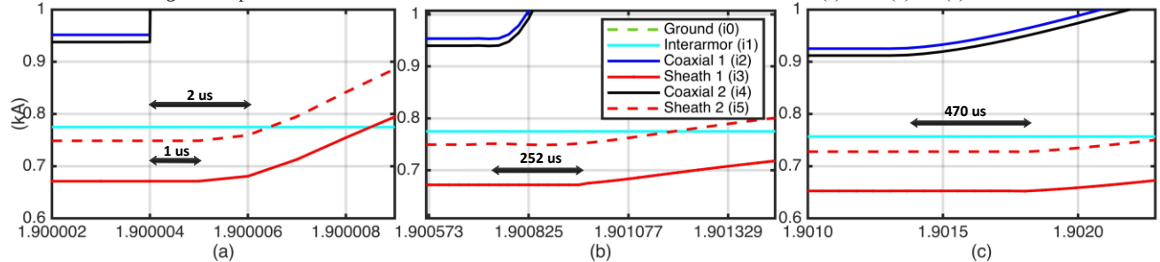
Fig. 11. Impact of fault distance on the modal fault location in TCE-HVDC cable. (a) 1 km (b) 150 km (c) 280 km
