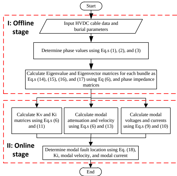
Fig. 7. Flowchart for calculating different parameters explained in section III. cable bundle. Tables II-V give modal characteristics based on different parameters. The results given in tables II-V are obtained in the frequency of 1 MHz. The highlighted values give the parameters used as the cable bundle data for fault localization in section V.
