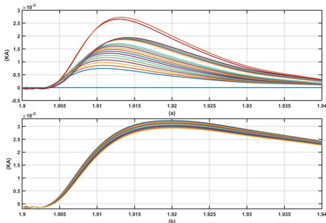
Fig. 13. Distributed ground currents in 20 ground points for TCE-HVDC cable (a) only armors grounded, (b) screen and armor connected together and then grounded.
