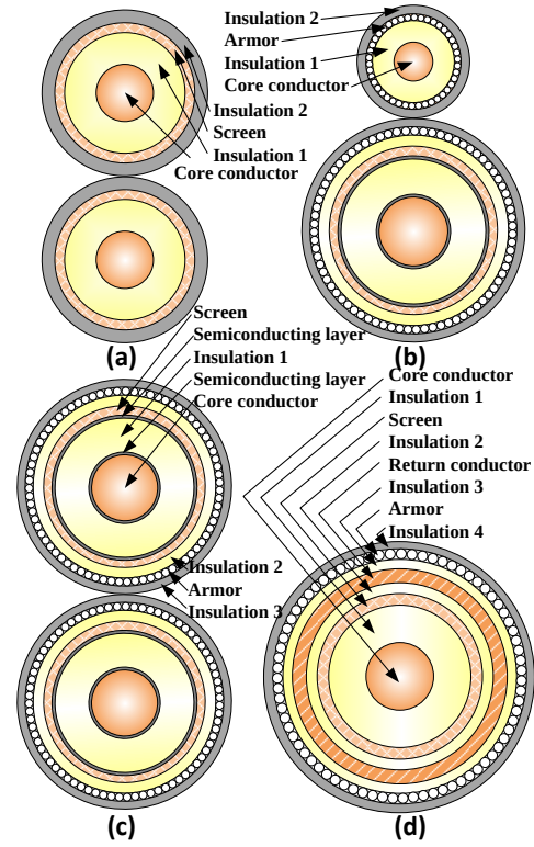
Fig. 1. HVDC cable bundles: (a) Two core coaxial (TCC-HVDC), (b) Single core extruded with metallic return (SCMR-HVDC), (c) Two core extruded (TCE-HVDC), (d) Extruded with integrated metallic return (EIMR-HVDC).
