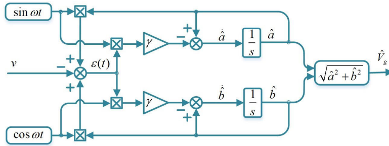
FIGURE 3. Proposed method for the amplitude estimation of the single-phase grid voltage.
