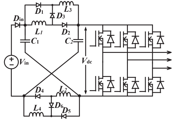
Fig. 2. Switched-inductor Z-source inverter [9].
