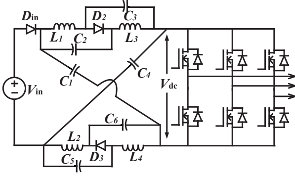
Fig. 3. MSC-ZSI topology [12].
