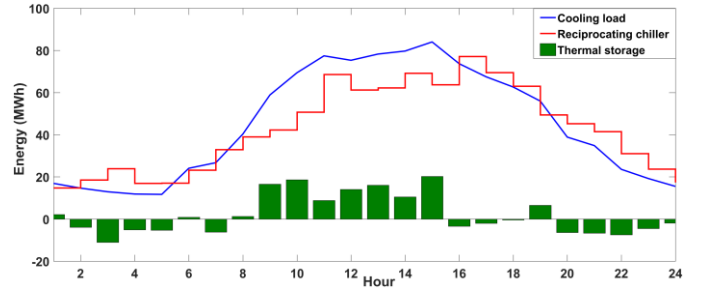
Fig. 4. The outputs of the RC unit and thermal storage during a day.
