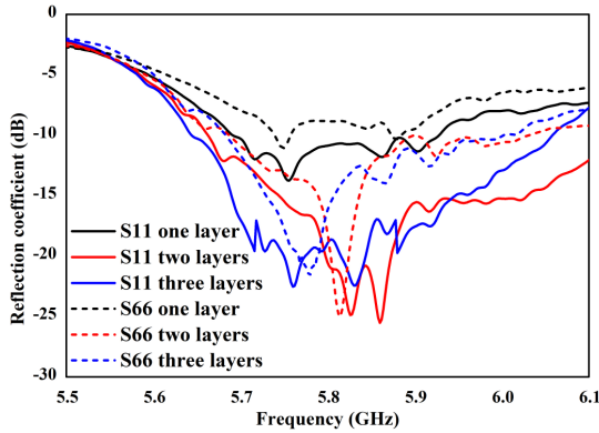
FIGURE 7. Reflection coefficients of proposed array with one layer of metasurface, proposed array with two layers of metasurfaces and proposed array with three layers of metasurfaces.
