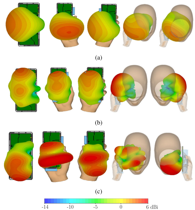
FIGURE 18. Directivity of antenna (a) 1, (b) 3, (c) and 4 when in free space, hold by the user hand phantom in data mode and in the presence of the user hand and head phantoms in talk mode.
