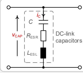
Fig. 6(a) Equivalent circuit of dc links
