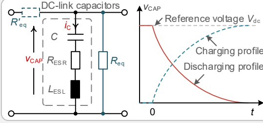
Fig. 6(b) Equivalent circuits and voltage profiles of RC charge and discharge schemes
