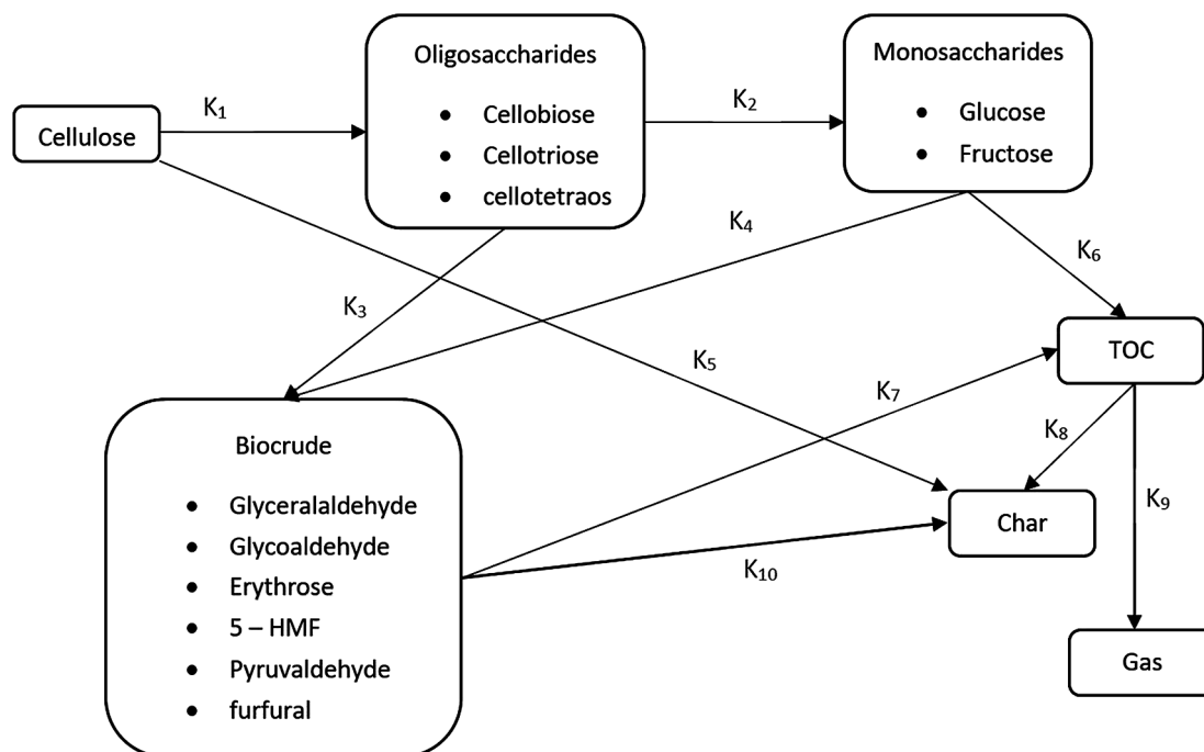
Fig. 2. Reaction pathway of cellulose decomposition.
