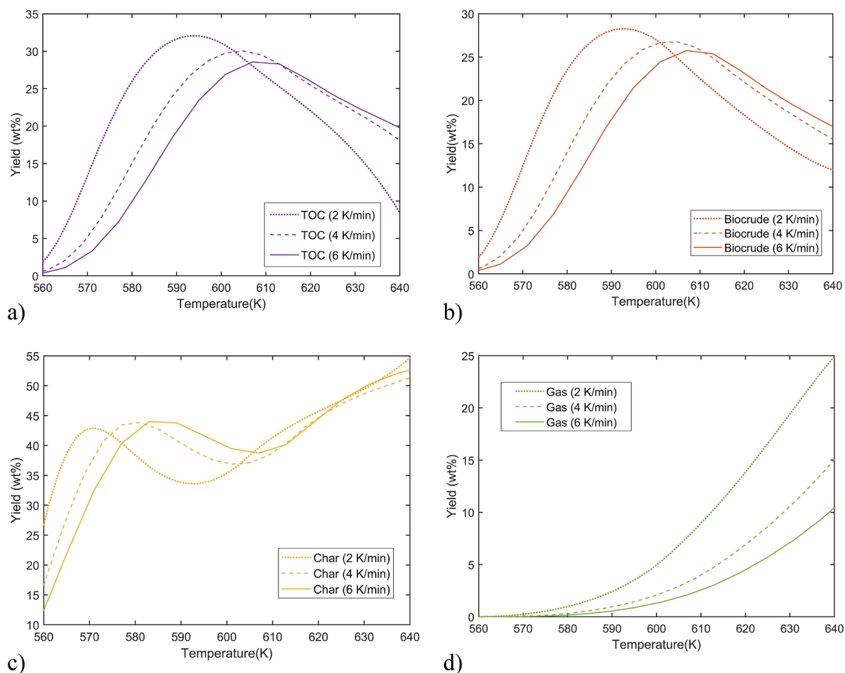
Fig. 10. Effect of heating rate on cellulose hydrolysis) TOC b) biocrude c) char d) gas.
