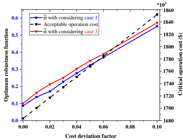
Fig. 25: Optimum robustness function with regard to deviation factor.
