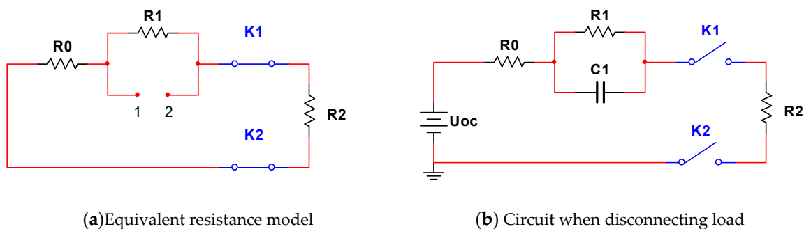
Figure 2. Equivalent circuit.
