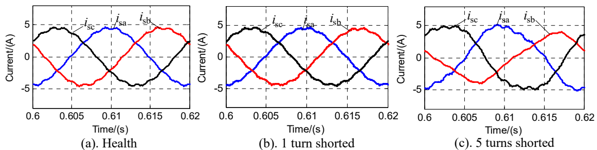
Figure 12. Currents of stator phases for R_f = 0.1 \Omega with different shorted turns.
