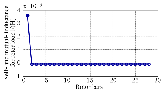
Figure 6. Inductances of the rotor loop 1.
