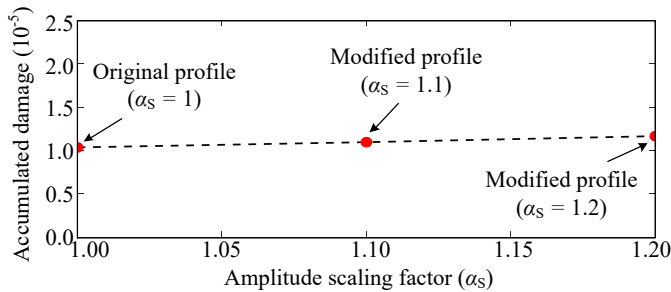
Fig. 16. Accumulated damage of capacitor under daily mission profile with different solar irradiance amplitude scaling factors (ambient temperature of T_a = 25 °C).
