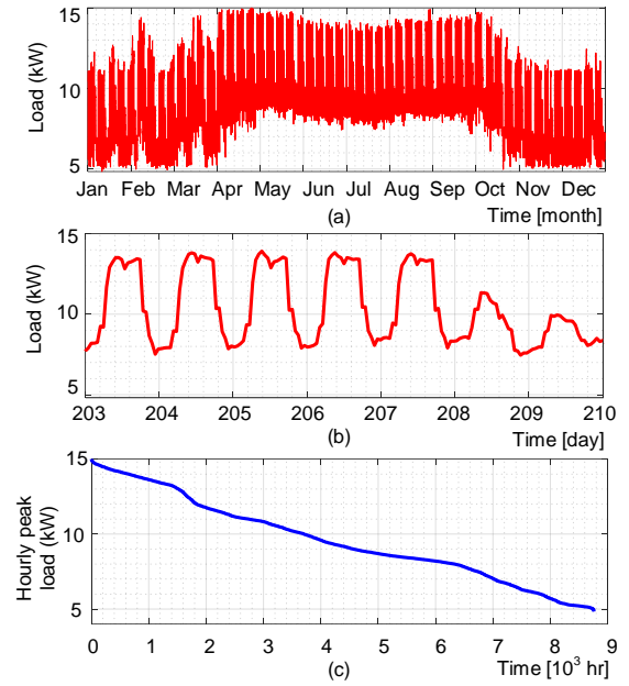
Fig. 8. Load profile for a small clinic; (a) annual load profile, (b) daily load profile for one week, and (c) load duration curve based on hourly peak load.
