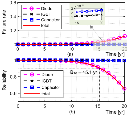
Fig. 12. Inverter wear out failure rate (a) and reliability (b).
