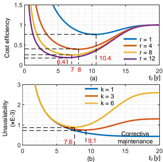
Fig. 18. Cost efficiency (a) and unavailability (b) of the capacitor bank in terms of planned replacement time t_0 .
