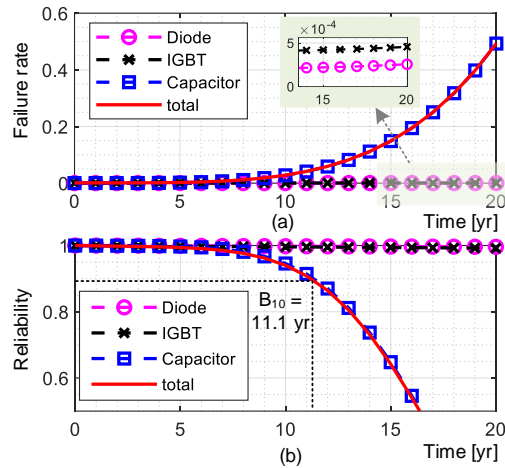
Fig. 10. PV converter wear out failure rate (a) and reliability (b).
