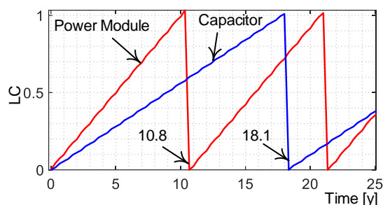
Fig. 20. Predictive maintenance based on LC: lifetime consumption.
