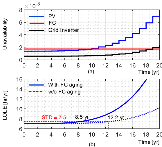
Fig. 15. Obtained system-level results showing the impact of FC converters aging: (a) individual generation unit unavailability and (b) LOLE– STD: standard level.
