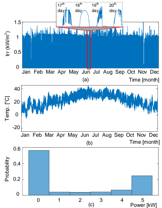
Fig. 9. Annual mission profiles: (a) solar irradiance, (b) ambient temperature, and (c) probability of PV system output power.
