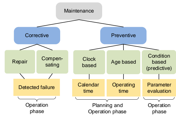
Fig. 4. Classification of maintenance types in a power system.
