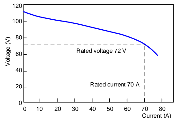
Fig. 7. Voltage-current characteristics of the Fuel Cell stack.
