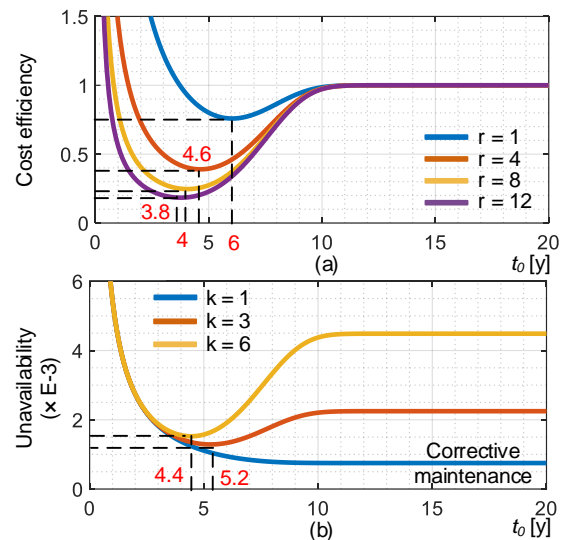
Fig. 19. Cost efficiency (a) and unavailability (b) of the power module in terms of planned replacement time t_0 .
