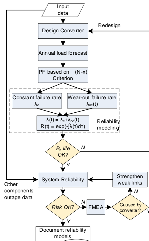
Fig. 3. System-level design for reliability in PEPS with N-x criteria – PF: power flow, FMEA: failure mode, and effect analysis.
