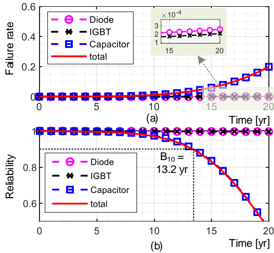
Fig. 11. FC converter wear out failure rate (a) and reliability (b).
