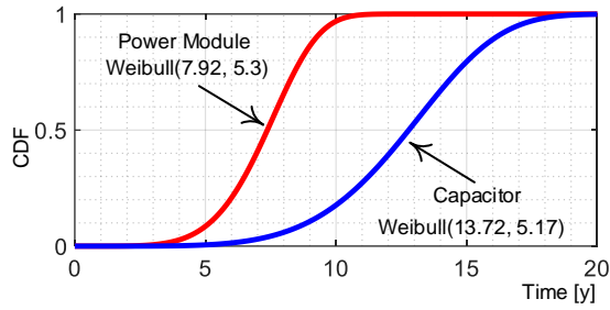
Fig. 17. Wear-out Cumulative Distribution Function (CDF) of power modules and capacitor bank for Case B.
