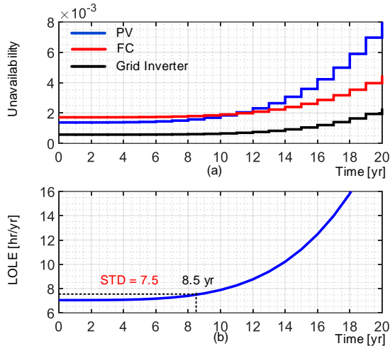
Fig. 13. Obtained system-level results: (a) individual generation unit unavailability and (b) LOLE – STD: standard level.
