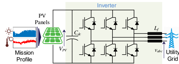
Fig. 16. Structure of a 100-kW central PV inverter for Case B.
