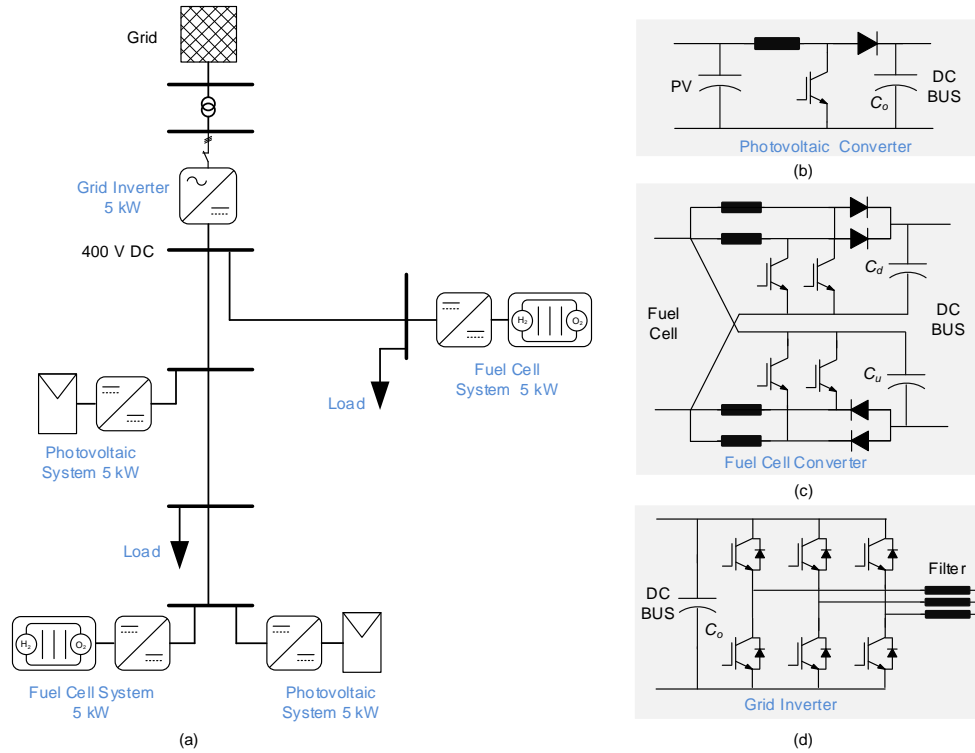
Fig. 6. Structure of dc Power Electronic-based Power System (PEPS); (a) single line diagram of the dc grid, (b) Photovoltaic (PV) converter, (c) Fuel Cell (FC) converter, (d) Grid inverter. (Case A)
