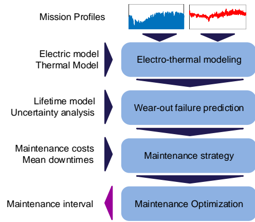
Fig. 5. Proposed age-based maintenance scheduling process in power electronic converters.
