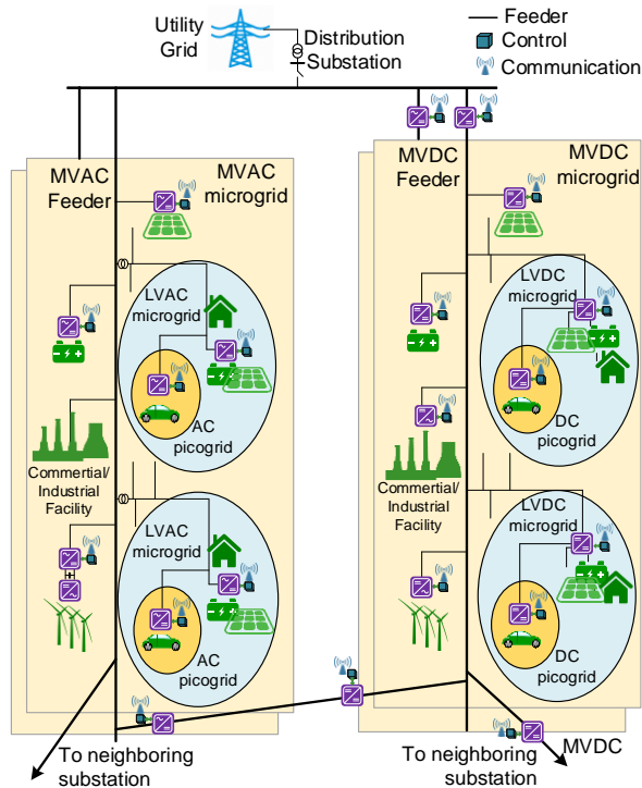
Fig. 1. Structure of future power electronic based power systems.
