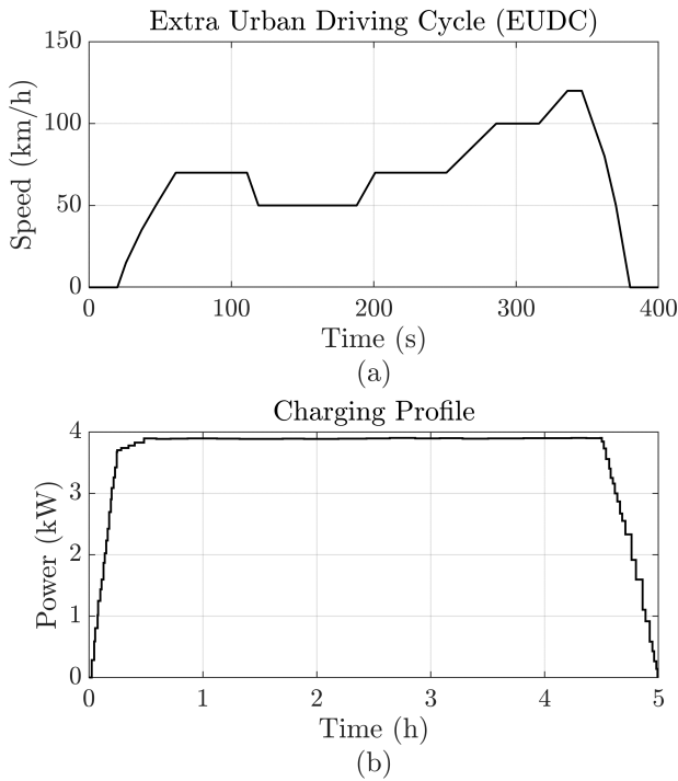
Fig. 8. Typical operational mission profiles for the two sub-assemblies (a) Electric vehicle driving cycle [80], and (b) Scaled-down power demand for an EV on-board charger (based on [81]).
