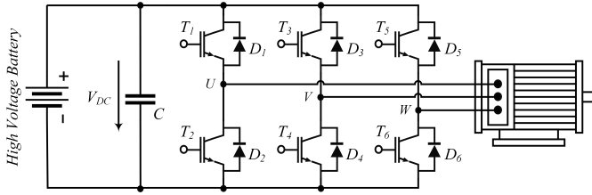
Fig. 4. Block diagram of standard voltage source inverter (VSI) topology used in the propulsion system.
