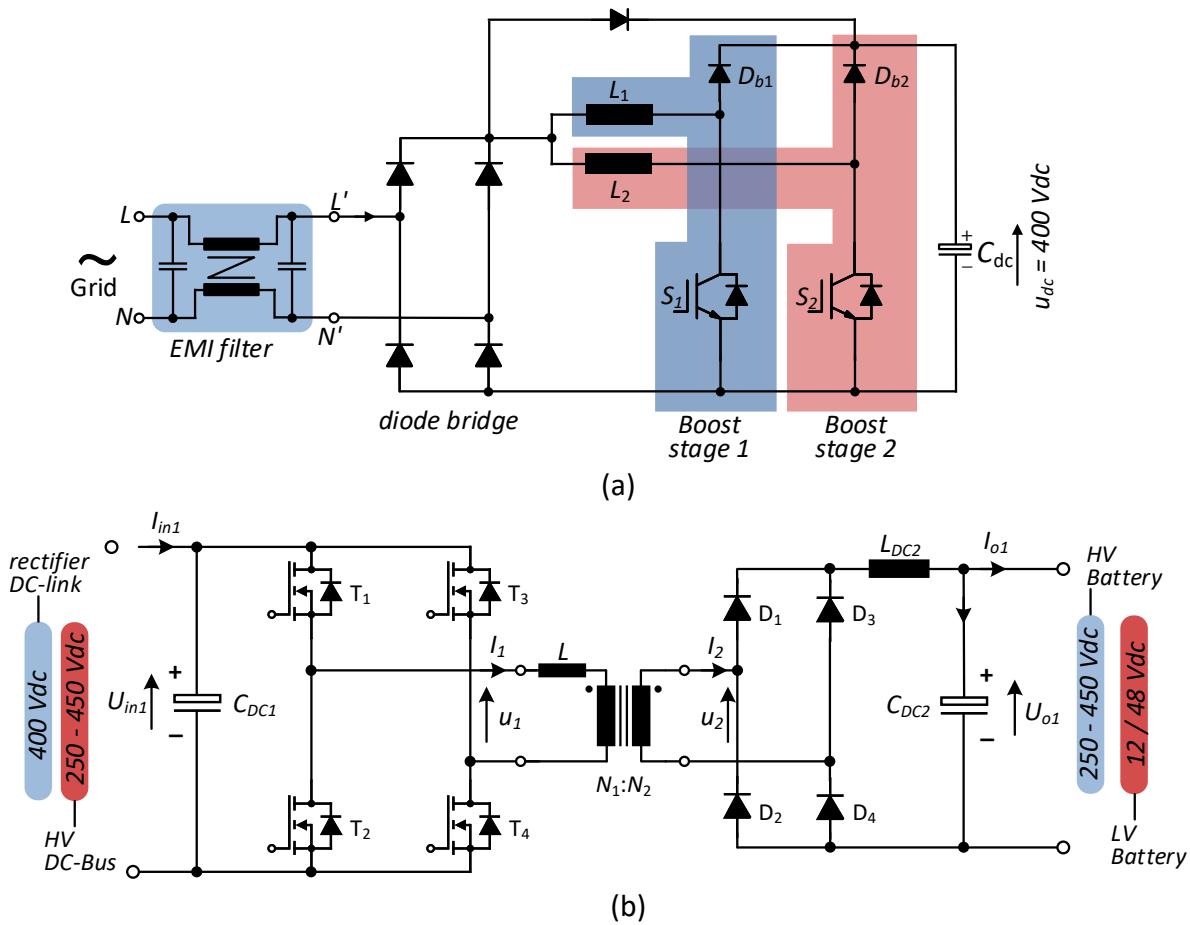
Fig. 3. Block diagram of on-board charger and DC-DC converters: (a) single-phase AC/DC with interleaved boost PFC topology, (b) isolated DC-DC converter with unidirectional phase shift full bridge (PSFB) configuration.
