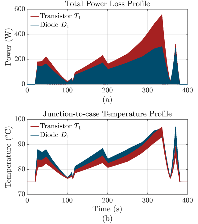
Fig. 10. Electro-thermal loading profiles of the drive train power semiconductor devices under the given mission profiles (a) Total power losses, and (b) Junction-to-case temperature for the drive train.
