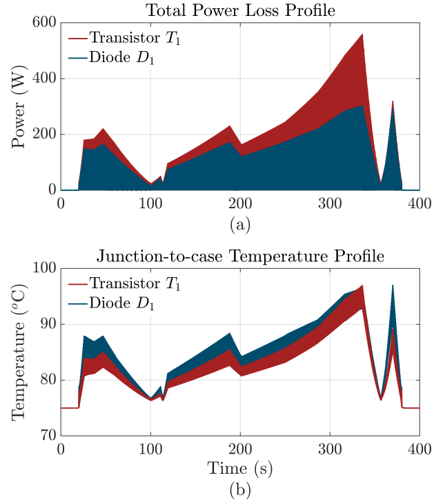
Fig. 10. Electro-thermal loading profiles of the drive train power semiconductor devices under the given mission profiles (a) Total power losses, and (b) Junction-to-case temperature for the drive train.
