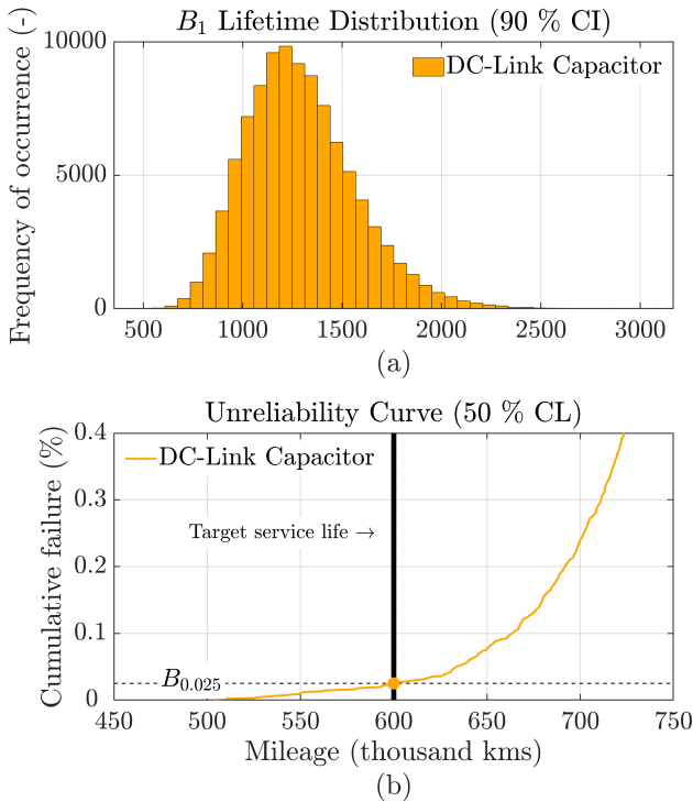
Fig. 12. Reliability metrics of the on-board charger DC-link capacitor (a) B 1 lifetime distribution with 90 % confidence interval (CI), and (b) Cumulative failure distribution of the B x lifetime with 50 % confidence level (CL).
