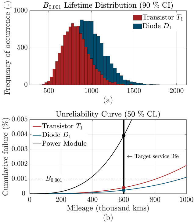
Fig. 11. Reliability metrics of the drive train IGBT power stage for the driving cycle (a) B_{0.001} lifetime distribution with 90 % confidence interval (CI), and (b) Cumulative failure distribution of the B_x lifetime with 50 % confidence level (CL).
