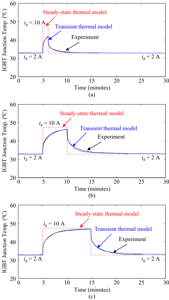
Fig. 4. Simulation and experimental results of thermal stress obtained from the transient and steady-state thermal models when the load dynamics (i.e., load durations) are: a) 1 minute, b) 5 minutes, and c) 10 minutes.
