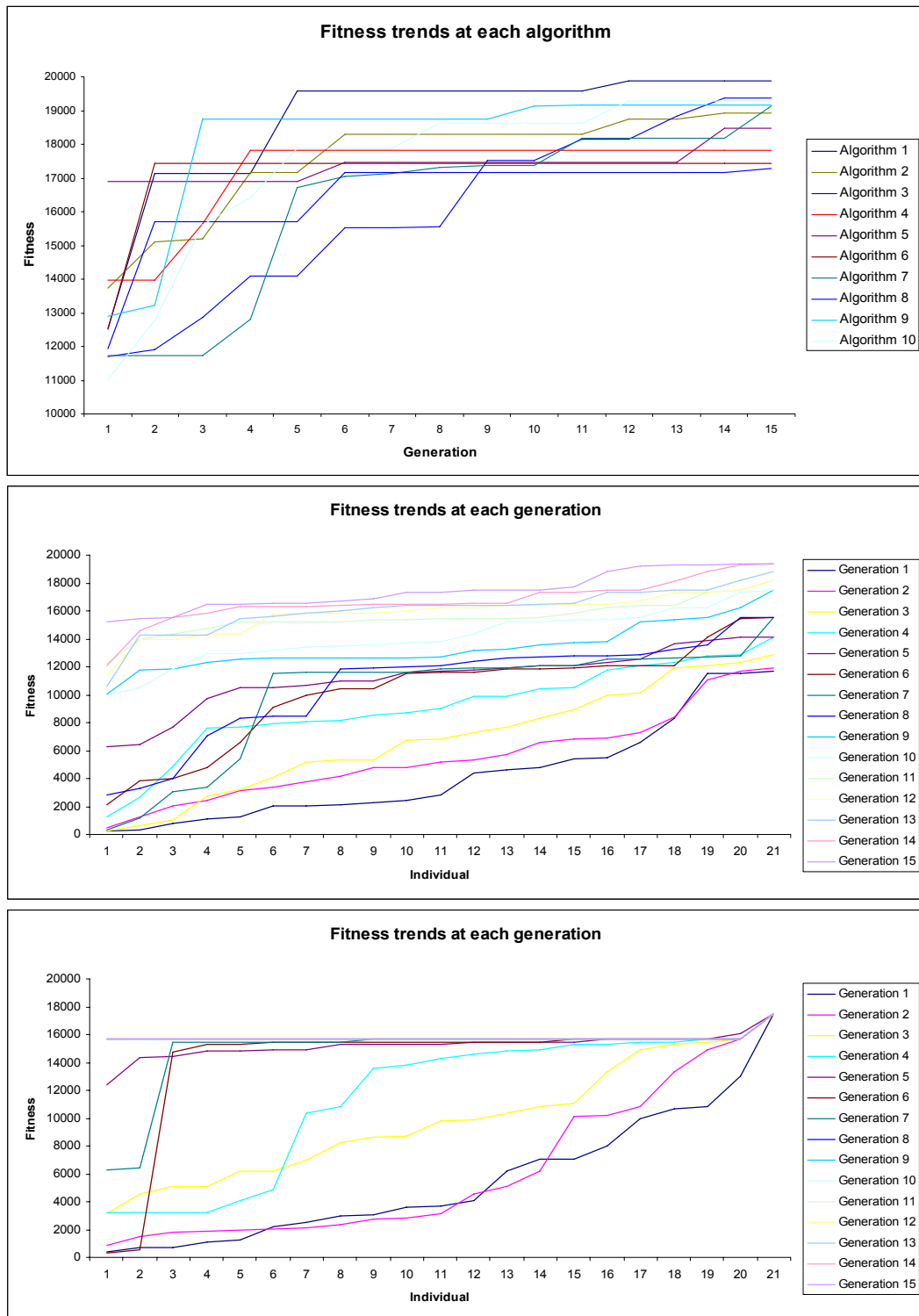
Figure 4 : Algorithm efficiency: best individual for each generation, crossover mutations, only crossover.
