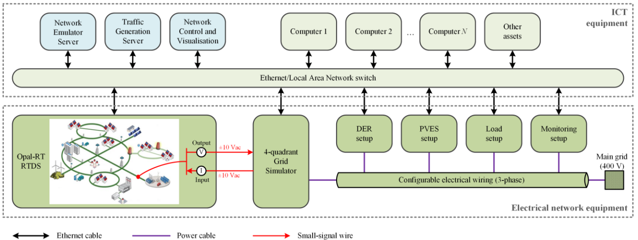
Fig. 2. Architecture of the laboratory platform for the study and testing of smart energy systems enabling-technologies
