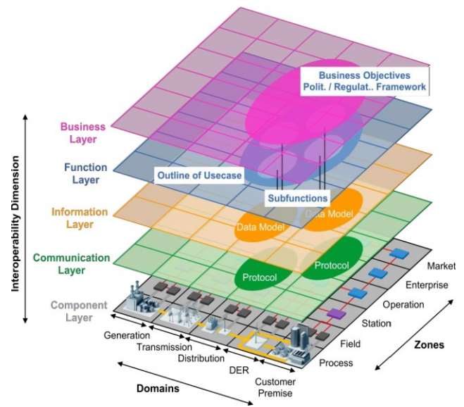
Fig. 1. SGAM framework [6]
