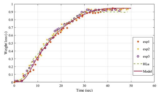
Fig. 6. Mass loss profile from model and experiment.
