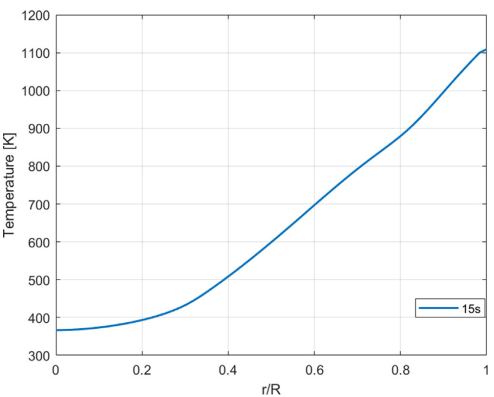
Fig. 16. Temperature along the pellet radius at 15 s.
