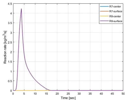
Fig. 13. Homogeneous reaction rate.
