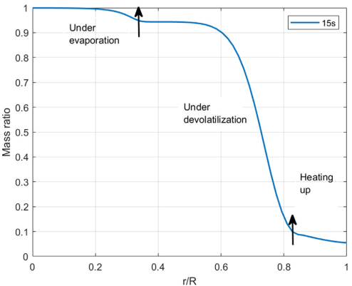
Fig. 18. Mass ratio along the pellet radius at 15 s.
