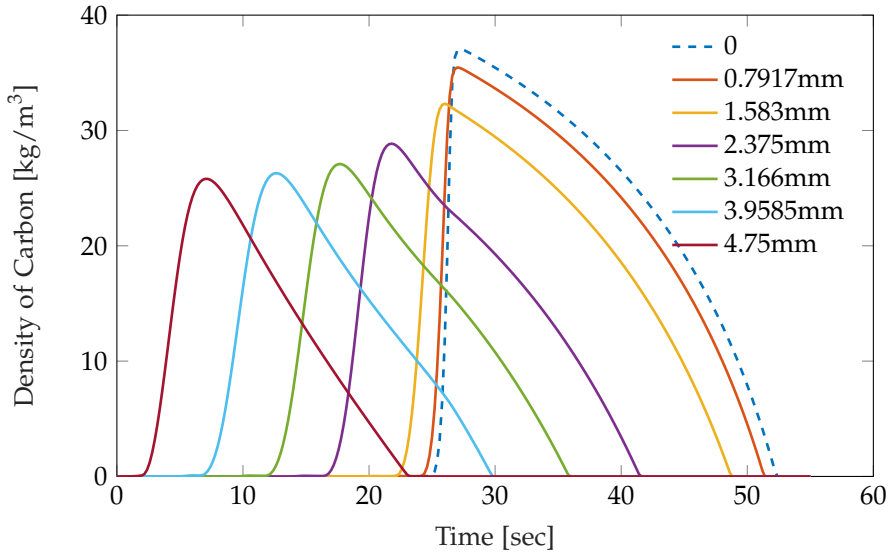
Fig. 3.6: Char density at different locations along the pellet radius
