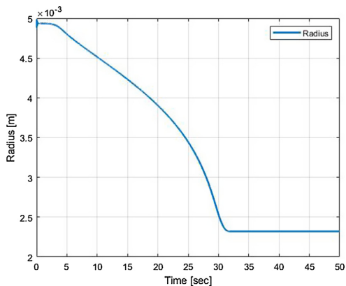
Fig. 15. Size changing during the pyrolysis process.
