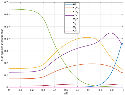
Fig. 17. Gas species along the pellet radius at 15 s.
