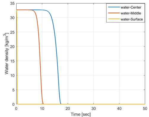
Fig. 8. Mass distribution of moisture within the pellet.
