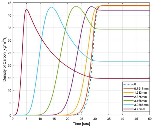
Fig. 4. Profile of carbon density within the pellet.
