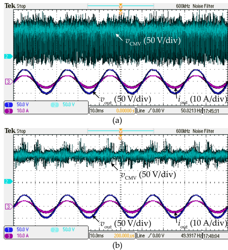
Figure 10. Experimental results of the CMV v_{cmv} , output voltage v_{out} and output voltage i_{out} when the RSPWM strategy, i.e., all even vectors in this paper, is used in (a) the conventional three-phase qZSI system and (b) the modified three-phase qZSI system [Time (10 ms/div)].
