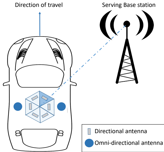
Fig. F.3: Antenna selection with the 6 directional antennas
