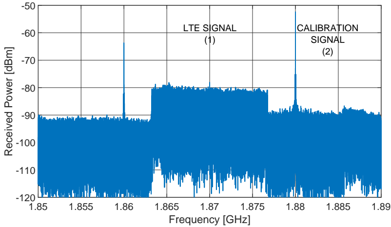
Fig. A.5: Received signal spectrum
