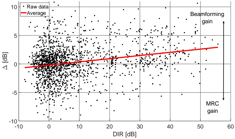
Fig. D.8: Dependence of DIR on receive beamforming gains
