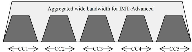
Fig. 1. Carrier aggregation of multiple continuous component carriers.
