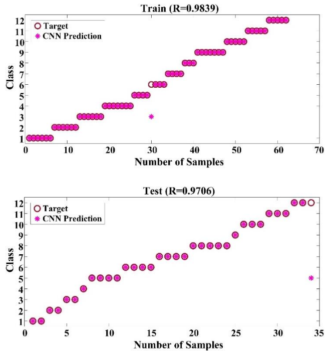
Fig. 10. CNN classification for the training and testing data of the REDD house 4 EAs
