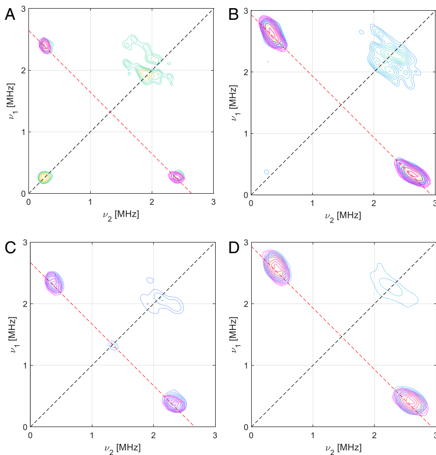
Fig. 4. ^{15}\text{N} -HYSCORE spectra and simulations of ^{63}\text{Cu} - ^{15}\text{N} - B /LPMO10A (A and B) and ^{63}\text{Cu} - ^{15}\text{N} - B /LPMO10A with squid pen \beta -chitin (C and D). Numerical simulations (in pink) were obtained with the values reported in Table 3. (A) ^{63}\text{Cu} - ^{15}\text{N} - B /LPMO10A near g_{\perp} with \tau = 136 ns at 3,995 G; (B) ^{63}\text{Cu} - ^{15}\text{N} - B /LPMO10A near g_{\parallel} with \tau = 136 ns at 3,060 G; (C) ^{63}\text{Cu} - ^{15}\text{N} - B /LPMO10A with squid pen \beta -chitin near g_{\perp} with \tau = 200 ns at 3,390 G; (D) ^{63}\text{Cu} - ^{15}\text{N} - B /LPMO10A near g_{\parallel} with \tau = 200 ns at 3,090 G.
