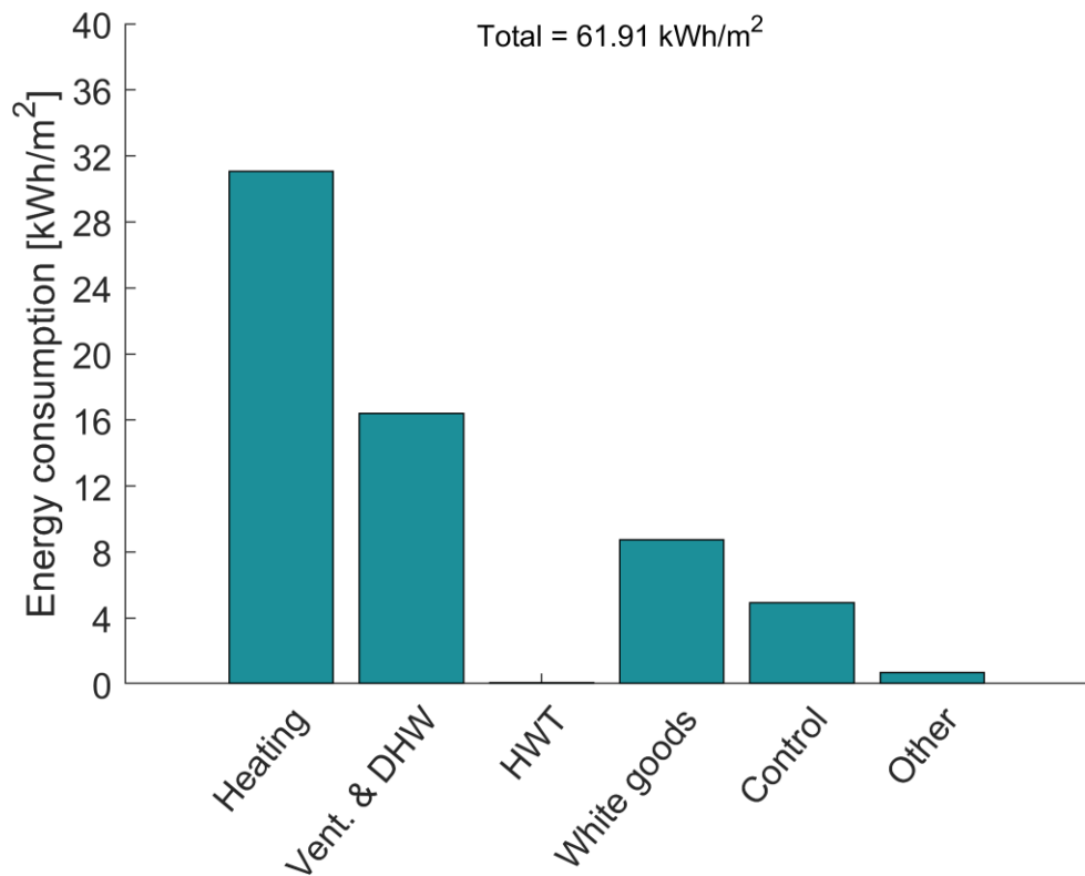
Figure 2.8: Yearly primary energy consumption for heating and electricity [kWh/m 2 ]
