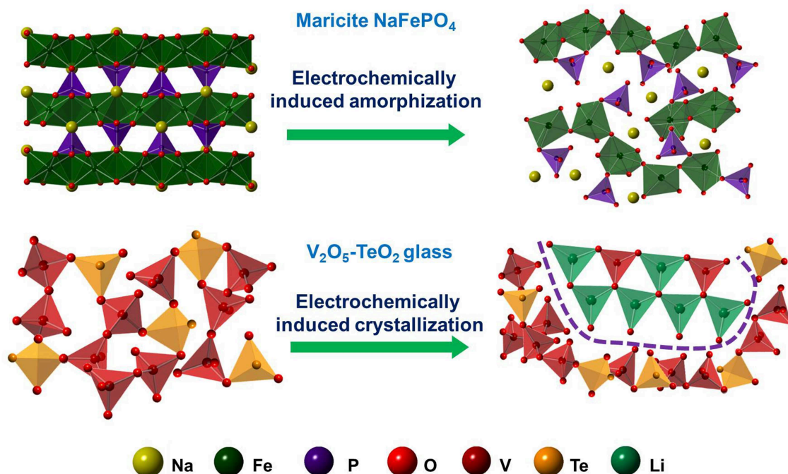
FIGURE 2 | Schematic diagram of structural evolution of electrochemically induced amorphization (maricite-type phase \text{NaFePO}_4 as an example) or crystallization ( \text{V}_2\text{O}_5 - \text{TeO}_2 glass as an example).
