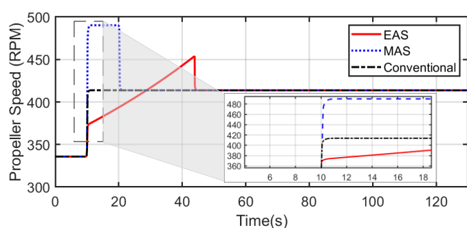
FIGURE 6. Actual and reference speeds of the propeller during an acceleration from 13 knots to 16 knots using different strategies of MAS, EAS and conventional.
