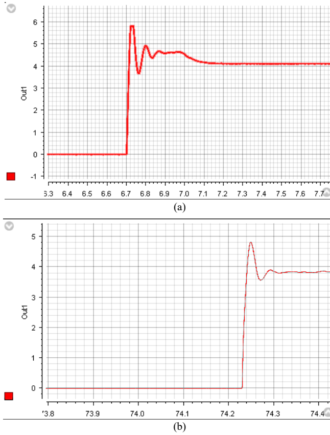
Fig. 36. The fault current of the LIED at one end of line for fault resistance of (a) 2 \Omega s with 2 km (b) 3 \Omega s with 1 km distance from LIED (Figure from JP4).
