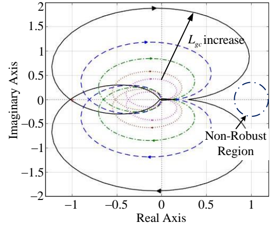
Fig. 10. Nyquist plots of \gamma(s) with different values of L_{gc} and a fixed R_d .
