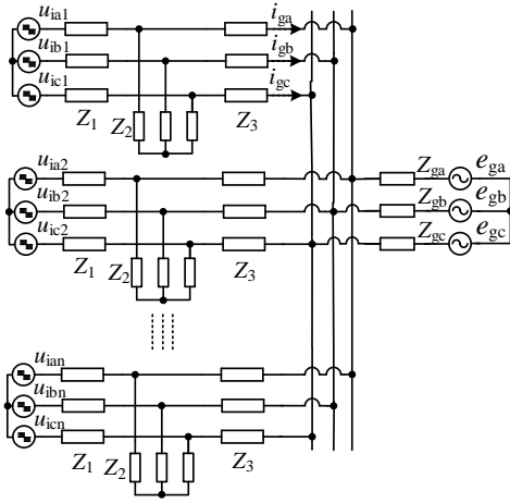
Fig. 5. The topology of N -paralleled grid-tied inverters.
