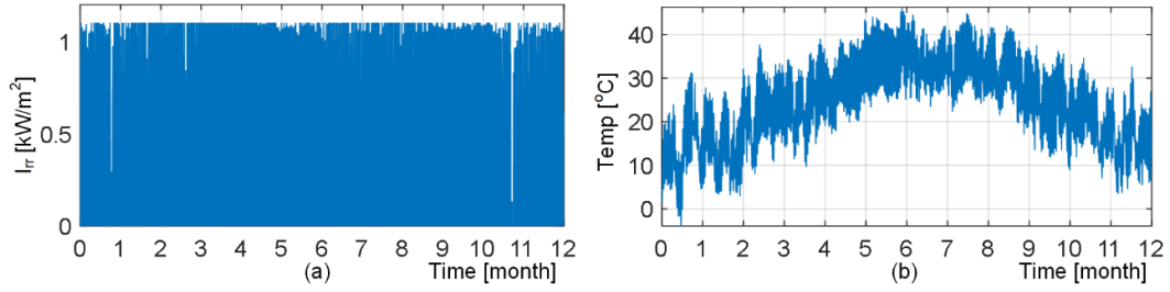
Fig. 5. Climate conditions for PV system: (a) solar irradiance ( I_{ir} ) and (b) ambient temperature (Temp).
