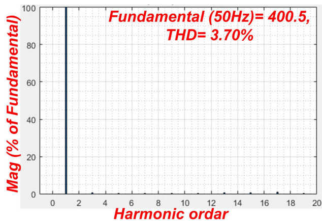
FIGURE 27. Simulation THD of 19 MLI.
