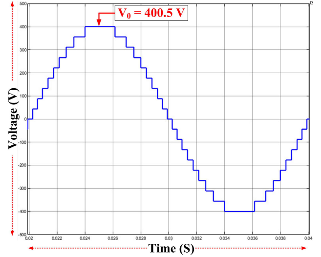
FIGURE 25. Simulation Phase Leg-A output waveform of 19 MLI.
