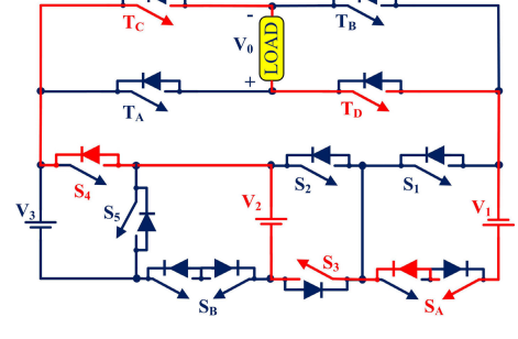
FIGURE 16. Mode-14 V_0 = -(V_1 + V_2) = -178V .
