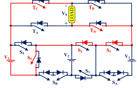
FIGURE 17. Mode-15 V_0 = -V_3 = -222.5V .
