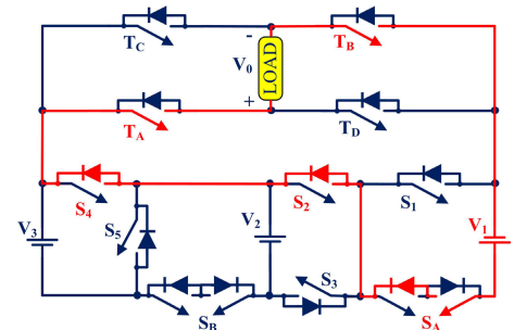
FIGURE 9. Mode-7 V_O = V_1 = +133.5V .
