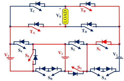
FIGURE 6. Mode-4 V_O = V_2 + V_3 = +267V .
