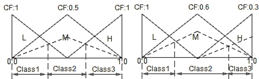
Figure 10. Membership linguistic variables boundaries with different CF.
