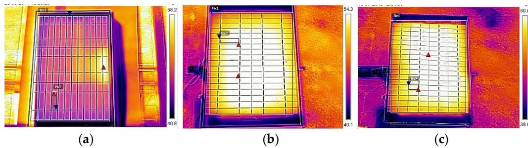
Figure 6. Modified thermal image of the PV panel under \Delta T^{\circ}\text{C} = 15^{\circ}\text{C} : (a) healthy, (b) EVA discolouring defect, (c) delamination defect.
