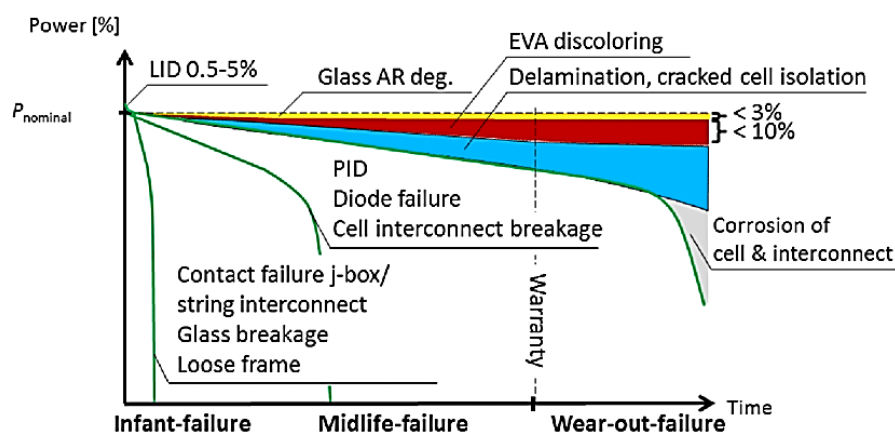
Figure 1. Power loss due to delamination and corrosion.
