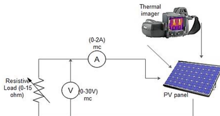
Figure 2. Schematic diagram of the experimental setup.
