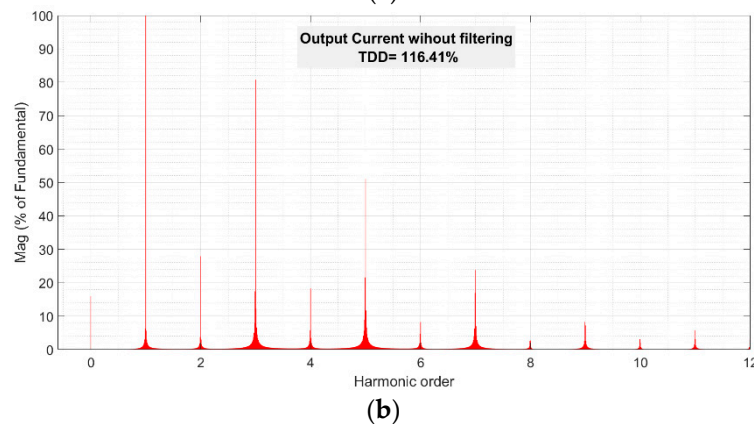
Figure 3. Scheme of a VSI with the existing approaches and the load’s distorted current: (a) block scheme of a single-phase VSI, showing the inner control loops of current and voltage, fed with the voltage reference generated by utilizing the Voltage Reference Generator block, based on References [45,53]; (b) nonlinear current harmonic distribution for Z_{NL} without filtering, after S_0 is turned on.
