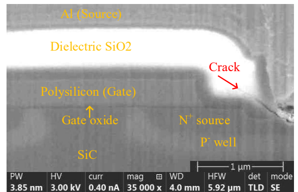
Fig. 1. Cross-sectional SEM image of the damaged cell. The red arrow identifies the SiO_2 dielectric crack [13].
