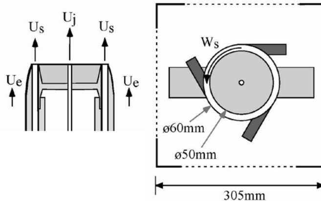
Figure 1: Structure of Sydney swirl burner
