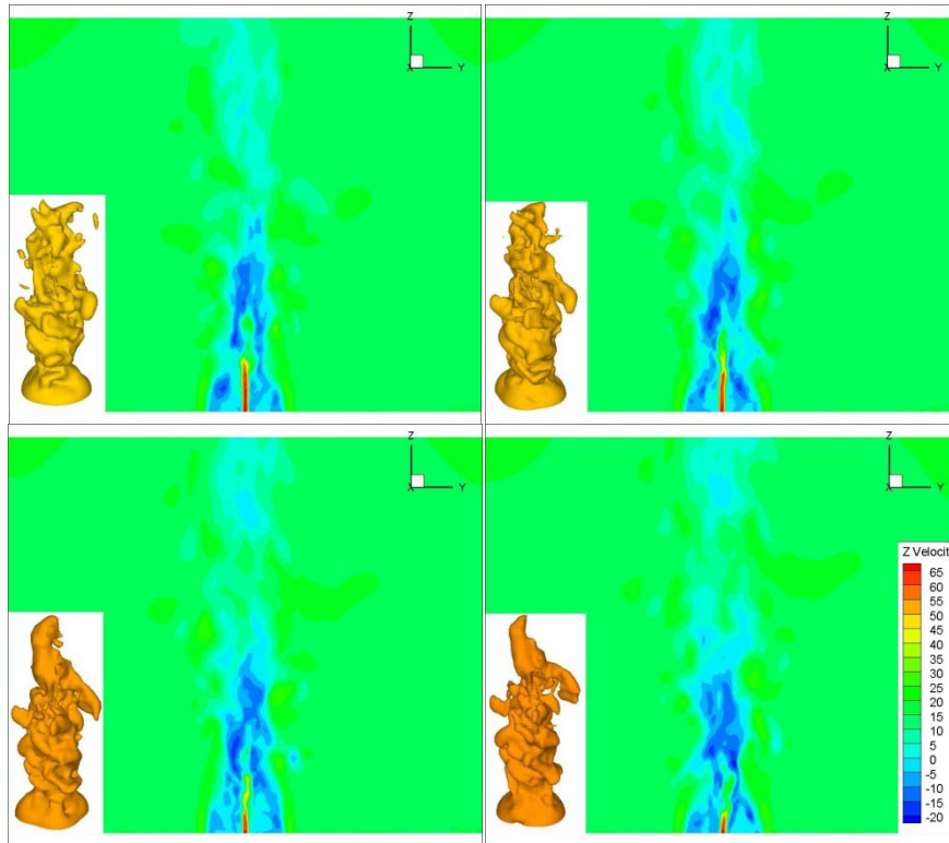
Figure 7: Isosurface of pressure and contour of axial velocity from t=0.171s to t=0.178s
