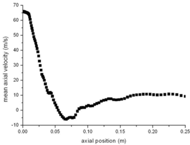
Figure 3: Mean axial velocity at centerline
