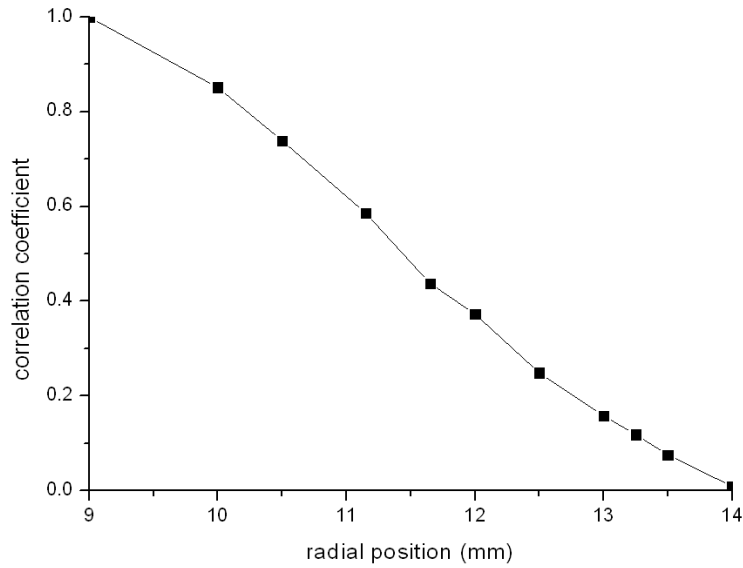
Figure 2: Two-point correlation coefficient at z=40mm, r=9~14mm
