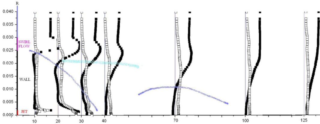
Figure 4: Radial distribution of average axial and relative RMS velocity along streamwise
