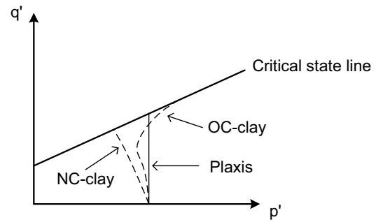
Figure 8: Effective stress paths for normally consolidated clay (NC-clay), overconsolidated clay (OC-clay) and for an undrained Mohr-Coulomb material with drained strength parameters defined in PLAXIS (Plaxis).
