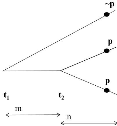
Figure 4: The Peircean model of branching time in which Fp is plainly false at the past moment t_1 , whereas it can be verified from the moment t_2 .
