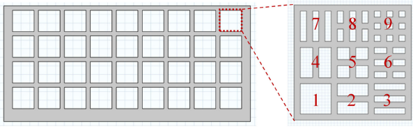
Fig. 7. Nine different cell patterns for each blank cell [3]. A GA is applied to determine the optimal combination of different cell patterns for the heatsink design for minimizing the junction temperature.
