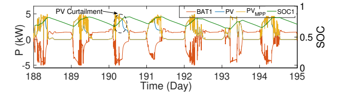
Fig. 14. Operating Conditions of PV and battery units in Case 1 for one week
