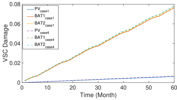
Fig. 20. Accumulated thermal damage progression over five years (Solid: 50 Hz thermal cycle; Dashed: Low-frequency included) in Case 4
