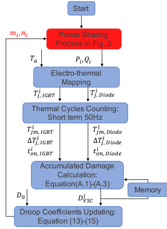
Fig. 4. The proposed process of droop gain adjustment for power sharing in an AC MG
