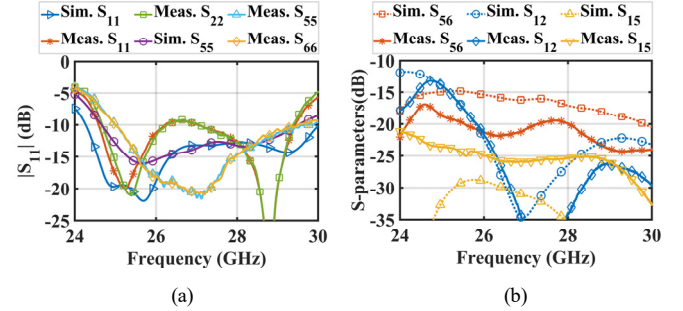
Fig. 9. The simulated and measured (a) reflection coefficients, and (b) mutual couplings of the presented antenna array.
