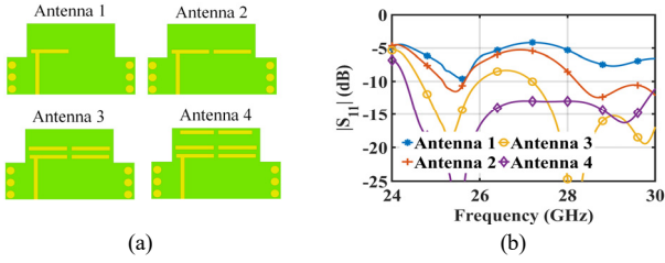
Fig. 5. (a) The design procedure of the H-mode, (b) The reflection coefficient comparison of different structures.
