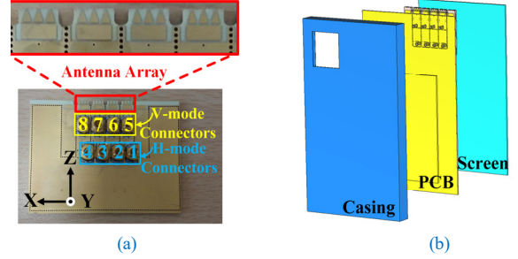
Fig. 8. (a) The fabricated antenna array. (b) Array inside the handset.
