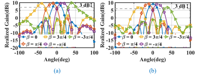
Fig. 10. The scanning performance of the presented antenna in the (a) H-mode, and (b) V-mode at 28 GHz.
