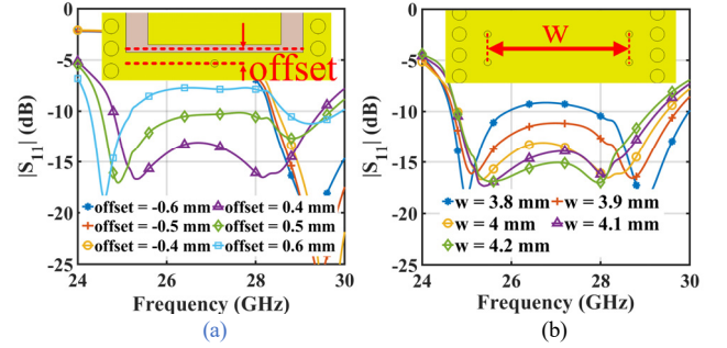
Fig. 3. The impact of the position of (a) center pin, and (b) side pins on the V-mode reflection coefficient.
