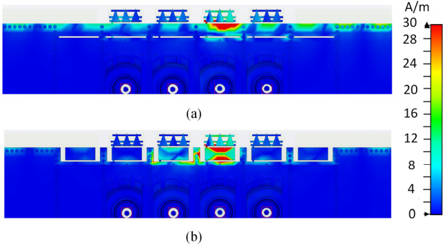
Fig. 7. The surface current distributions: (a) without z-oriented slots and (b) with z-oriented slots at 28 GHz.
