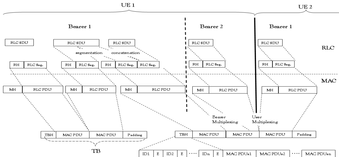
Figure 3: Proposed solution for user multiplexing in LTE-Advanced.
