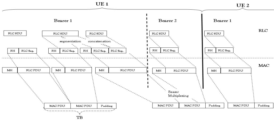
Figure 2: Data flow in the protocol stack in LTE Release 8.
