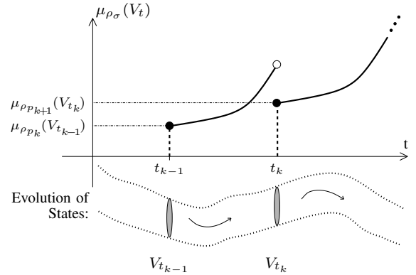
Fig. 5. The change of integrals of densities with time.
