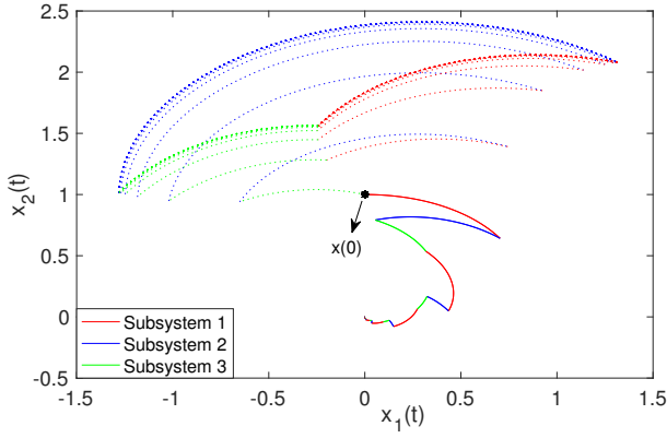
Fig. 1. A solution of Example 1. The dotted line is for the backward solution, which approaches to a limit cycle as t \rightarrow -\infty . The solid line is for the forward solution, which approaches to \mathbf{0} as t \rightarrow \infty .
