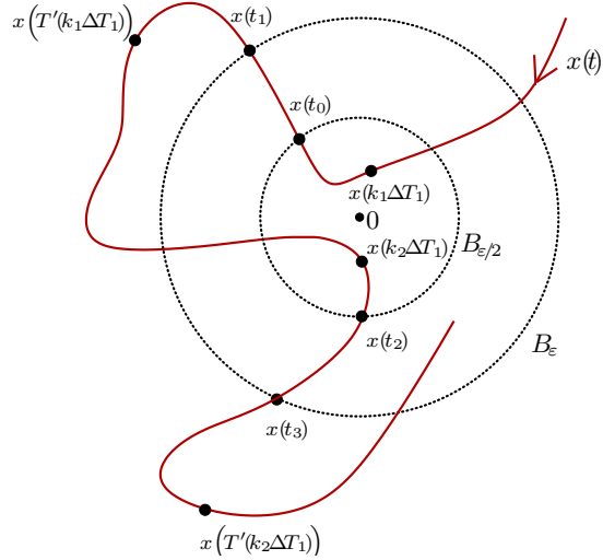
Fig. 3. An illustration for the proof of Lemma 3.
