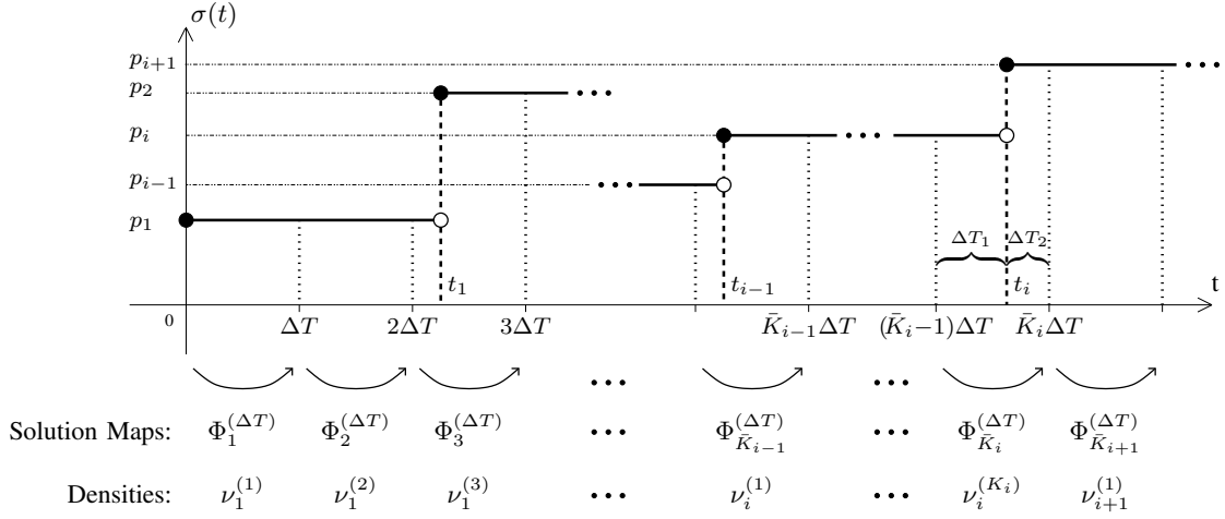
Fig. 4. An illustration for the proof of Lemma 6.
