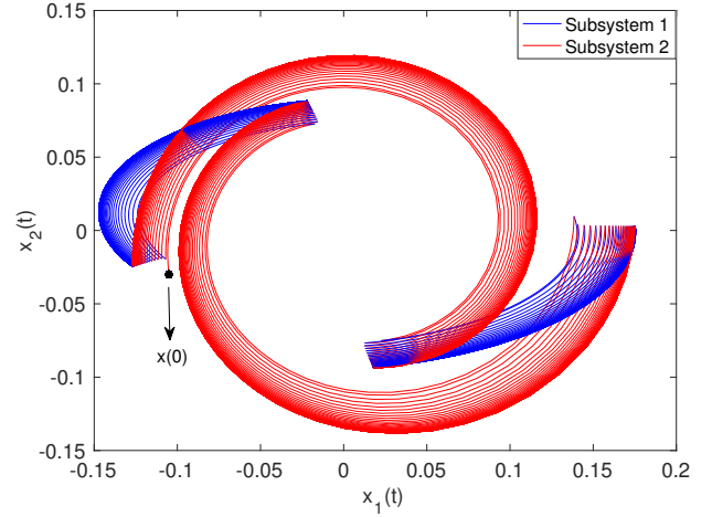
Fig. 2. A solution of Example 2 for the switching signal \sigma(t) = ((1, 4.7), (2, 1.7)) that does not satisfy the dwell time condition \tau > 5.7762 . The solution approaches to a limit cycle.
