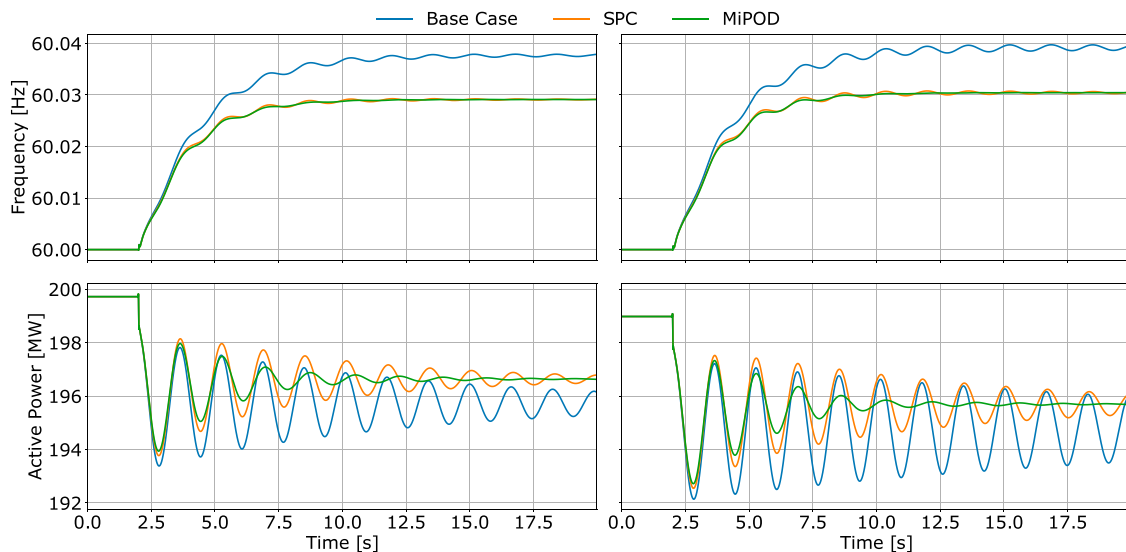
FIGURE 16 | System frequency and active power flow at B08 after a sudden 5% increase of reactive power demand by L9 for 2 random operating points.
