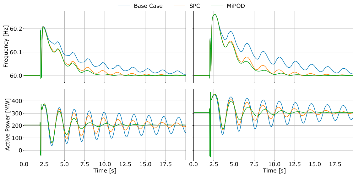
FIGURE 19 | System frequency and active power flow at B08 after a symmetrical fault at B07 for 2 random operating points while the lower line connecting B08 and B09 is out of service.
