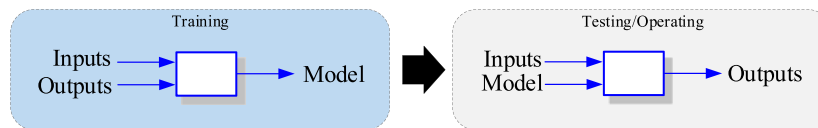
FIGURE 6 | Conceptual representation of Supervised Learning.
