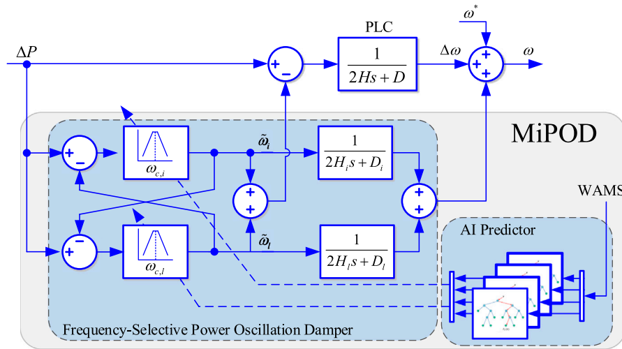
FIGURE 3 | Control block diagram of the MiPOD.
