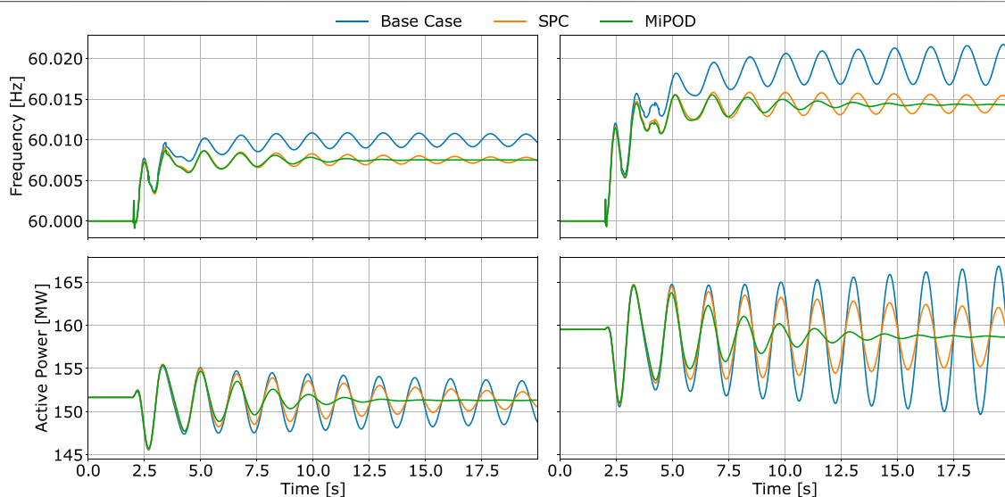
FIGURE 18 | System frequency and active power flow at B08 after a sudden change in the mechanical torque of G3 and G4 for 2 random operating points.
