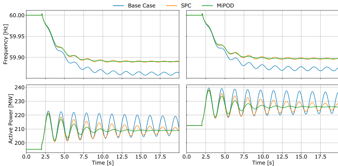
FIGURE 17 | System frequency and active power flow at B08 after a sudden 5% increase of active power demand by L9 for 2 random operating points.
