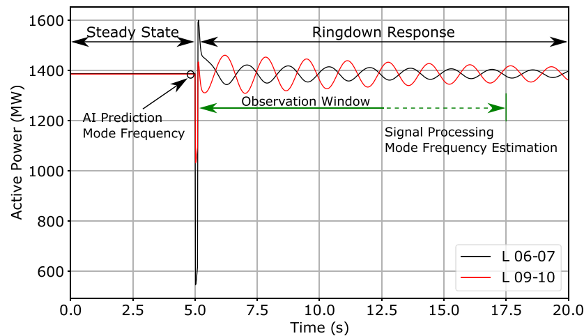
FIGURE 5 | Comparison between the proposed AI-based mode estimation approach and the traditional signal processing techniques. A properly trained AI model can provide fast and accurate estimations of the mode frequency faster than signal processing.
