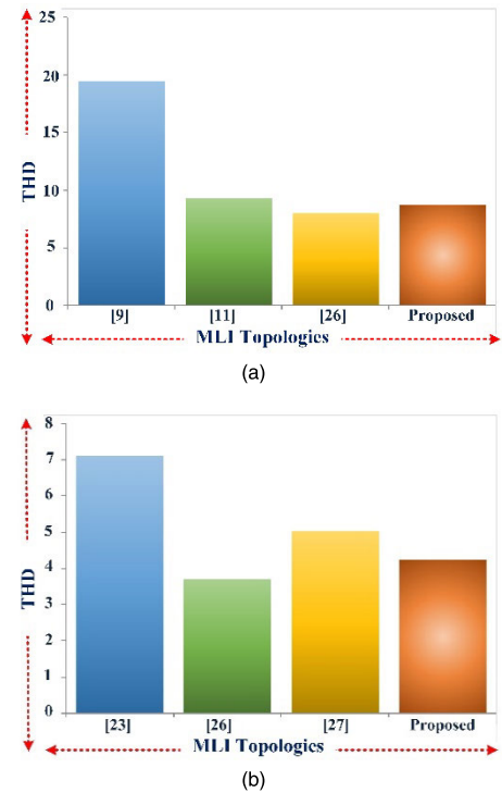
FIGURE 23. Comparison of THD (a) Proposed 9MLI with other topologies and (b) Proposed 17MLI and other similar topologies.
