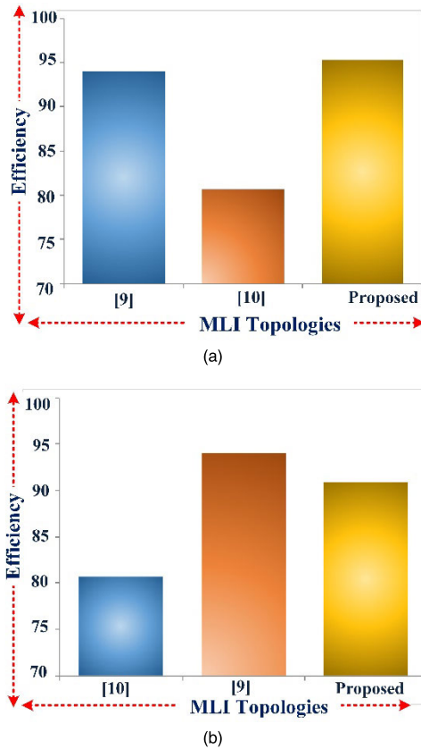
FIGURE 22. Comparison of efficiency to the proposed inverter with other topologies (a) 9 Levels (b) 17 Levels.
