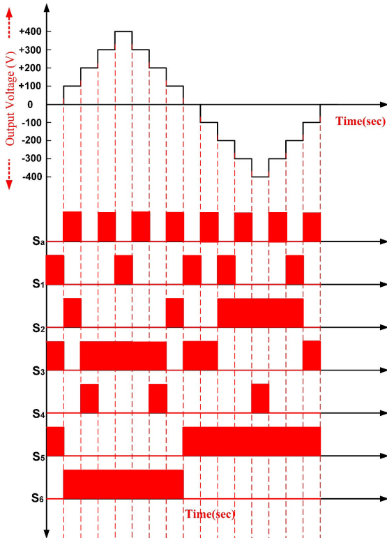
FIGURE 3. Expected 9 level waveform of the proposed topology proposed.
