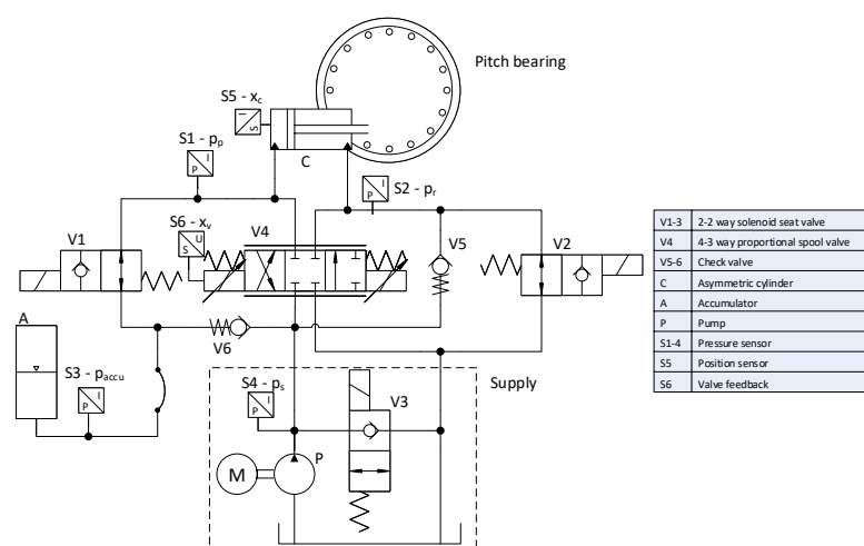
Figure 1. Simplified example of fluid power pitch system.
