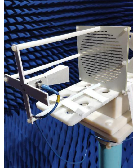
Fig. 14. Measurement setup of the proposed reflectarray.
