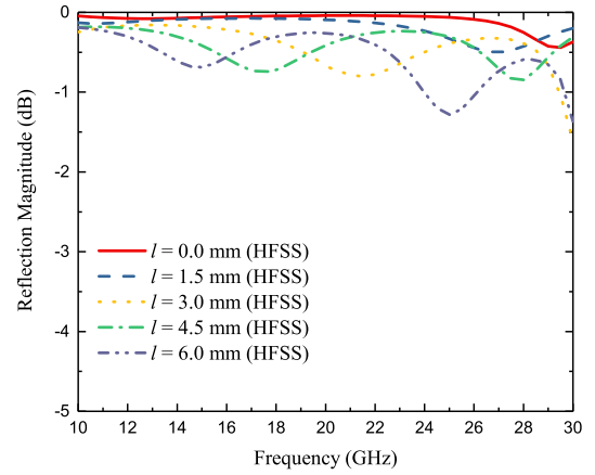
Fig. 6. Reflection magnitudes of the unit cell with different l .
