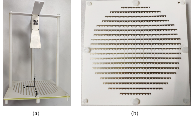
Fig. 13. Prototype of the proposed reflectarray. (a) Perspective view. (b) top view of the array aperture.
