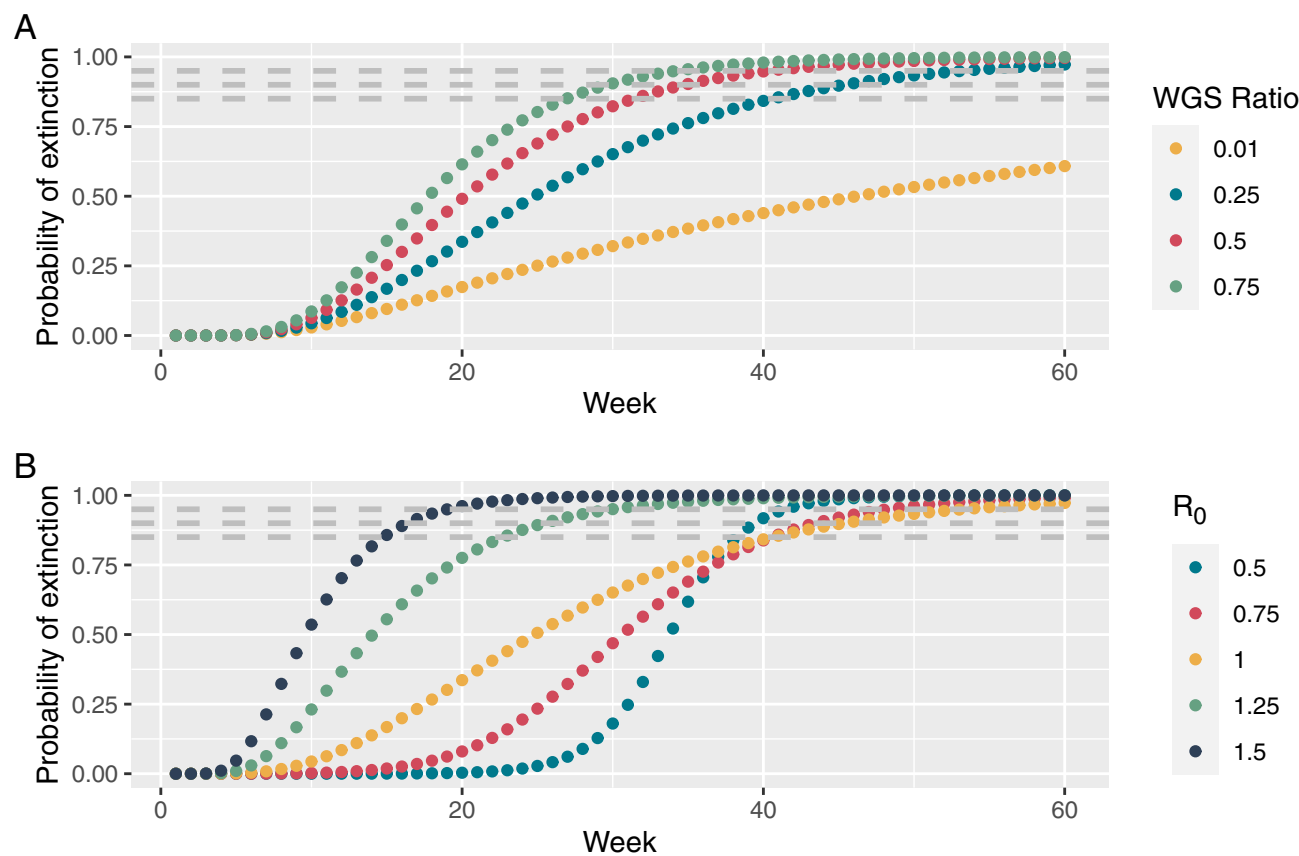
Figure 1. Probability of extinction as a function of the number of weeks with no observations of the specific variant. Dashed lines indicate probability levels 0.85, 0.90, and 0.95, respectively. (A) Variation of testing regime for a constant reproduction rate of R_0 = 1 . (B) Variation of restrictions ( R_0 ) for a constant WGS testing ratio of 0.25. The blue curve in upper plot is the same as the yellow curve in the lower plot.
