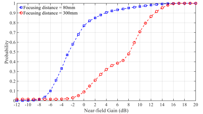
Fig. 7. The calculated CDFs of near-field gain of near-field focusing RISs with assigned focal distances of 80 and 300mm.
