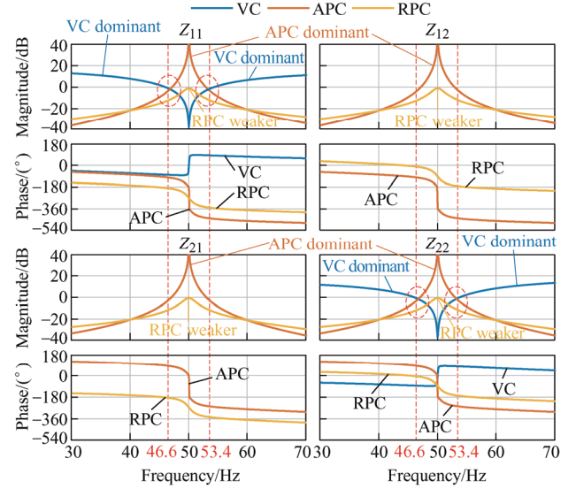
Fig. 8 Bode diagrams of \mathbf{Z}_o , \mathbf{Z}_{\text{ref}}\mathbf{G}_{\text{vv}} , and \mathbf{Z}_{\text{ref}}\mathbf{Q}\mathbf{G}_{\text{vv}}
