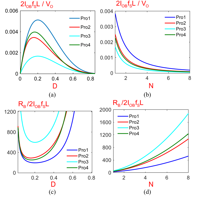
FIGURE 7. Normalized boundary conduction mode output current with respect to: (a) duty cycle in N_2 = N_3 = N = 3 , and (b) turns ratio in D = 0.6 . Normalized load resistance with respect to (c) duty cycle in N_2 = N_3 = N = 3 , and (b) turns ratio in D = 0.6 .
