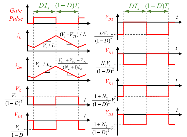
FIGURE 4. Typical voltage and current waveforms of Pro4 in CCM operation.
