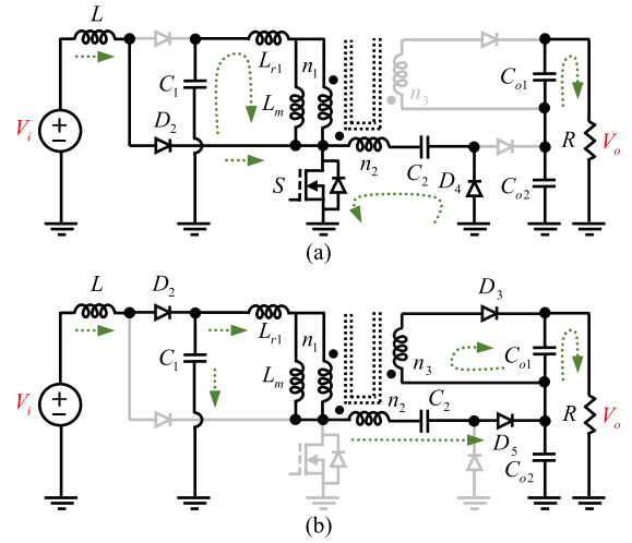
FIGURE 3. Equivalent circuits of Pro4 in; (a) Mode 1. (b) Mode 2.
