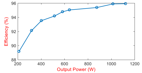
FIGURE 16. Efficiency with respect to the output power.
