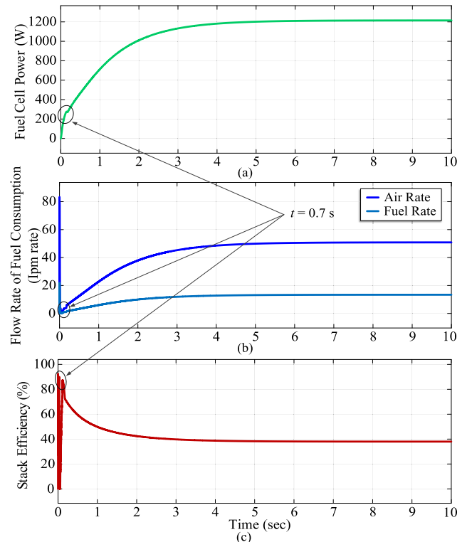
FIGURE 14. The operation outputs of the fuel cell system during 10 seconds; (a) the power of the fuel cell, (b) flow rate of fuel consumption in terms of insertion paddlewheel meter (lpm), and (c) stack efficiency of the fuel cell system.
