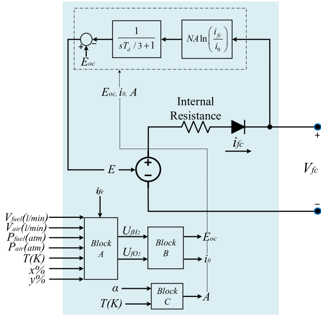
FIGURE 5. Detailed fuel cell model.
